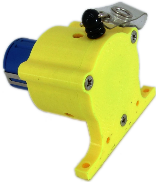
Assembled Version using modified FRC Team 2468 3D Print Files
